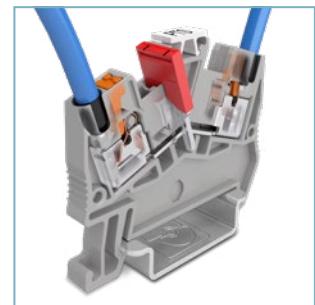
Bauform PTS
