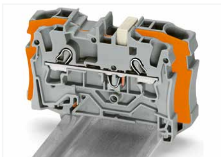
Step-down jumper (Item No. 2006-499) commons 6/4 mm 2 (10/12 AWG) terminal blocks (2006/2004 Series) with 4/2.5/1.5 mm 2 (AWG 12/14/16) terminal blocks (2004/2002/2001 Series).
