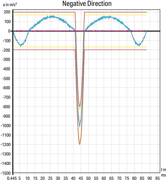
Time-Dependent Course of the Shock / 100 g, 6 ms Negative Direction
