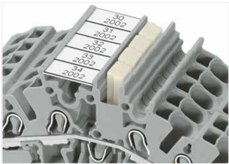
Adjacent jumpers for continuous commoning (Item No. 2002-400)
