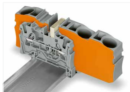
Step-down jumpers (2006-499 and 2016-499)
