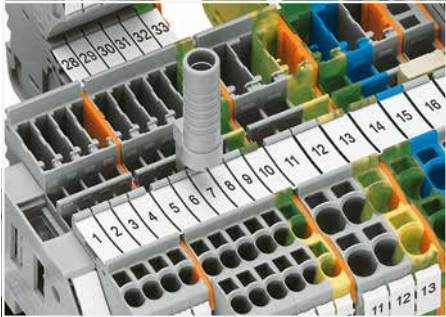
Test plug adapter (Item No. 2009-174) for 4 mm test plugs or banana plugs – also suitable for X-COM®S-SYSTEM-MINI Terminal Blocks.
