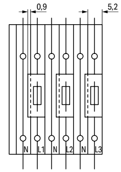
Open side of terminal block left
