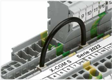
Commoning with push-in type wire jumper.
