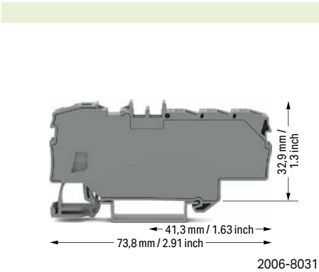
A clear marking of clamping units is molded in.
