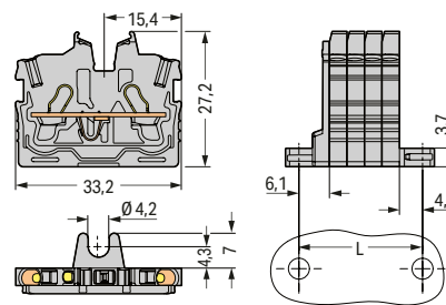
Modular Terminal Blocks and Terminal Strips with Mounting Flanges L = (Pole no. x 3,5 mm) + 4,3 mm + 6,1 mm
