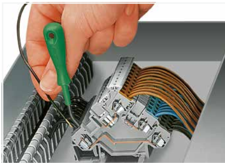
This operating tool with blade dimensions per DIN 5264 is ideal for front-entry sensor/actuator terminal blocks (280 Series).
