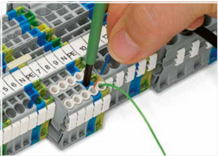
Inserting a conductor into the insulation stop.
