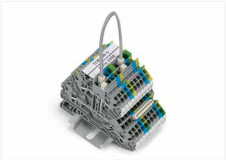
Push down the wire jumper until fully inserted. For rewiring, lift the jumper with an operating tool at the notch provided for this purpose on the jumper.
