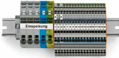
TOPJOB® S FI/LS main distribution board set; with operating slots
