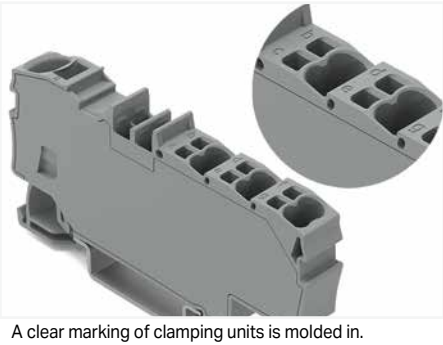
A clear marking of clamping units is molded in.
