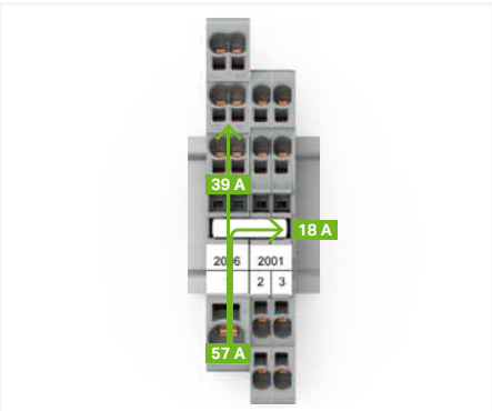
Commoning options for the 2006 Series Distribution Terminal Blocks and 2001 Series Terminal Blocks using 2001 Series Jumpers
