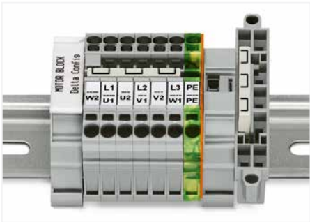
This delta jumper has been specially developed to create a delta configuration and is used on motor terminal boards equipped with TOPJOB® S rail-mount terminal blocks.
