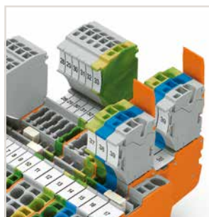
Female plugs can be individually locked.
