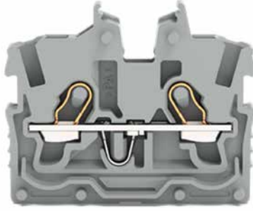
Through terminal block
