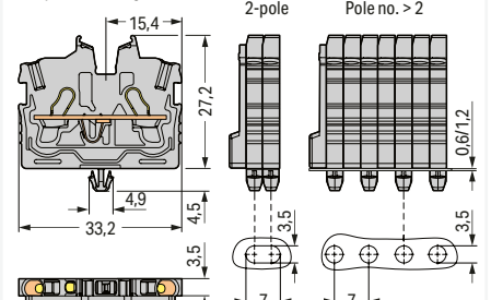
Modular Terminal Blocks and Terminal Strips with Snap-in Mounting Feet
