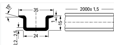
Copper DIN-rail ▶ I N 309 A (based on 1 m length) ▶ 35 x 15 mm ▶ 2.3 mm thick ▶ 2 m long ▶ per EN 60715
