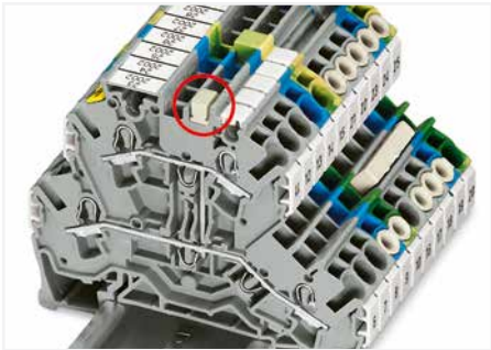
Commoning two levels via double-deck vertical jumper (Item No. 2002-492).
