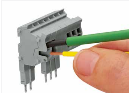
Conductor termination via: Operating tool for fine-stranded conductors without ferrules Push-in connection of solid conductors
