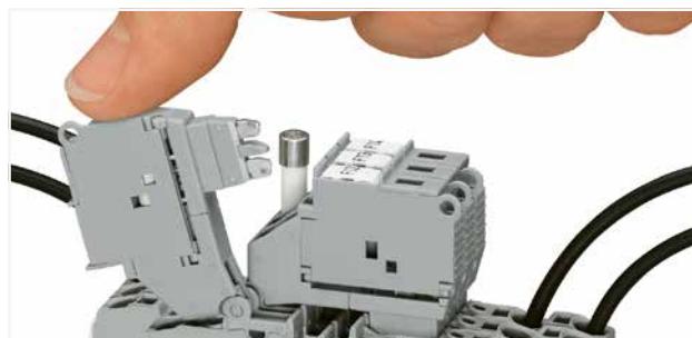
Pivot the fuse holder into the locked open position. Fuse terminal blocks for miniature metric fuses are rated at 2.5 mm 2 (12 AWG) and 6 mm 2 (8 AWG).
