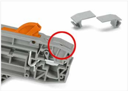
Lockout cap (2006-191) seals unused conductor entry.
