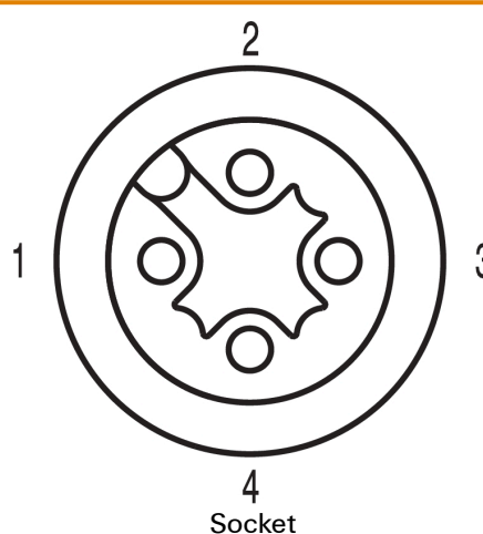
Angled socket
