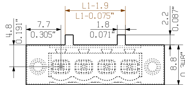
FRONT PLATE CUT-OUT
