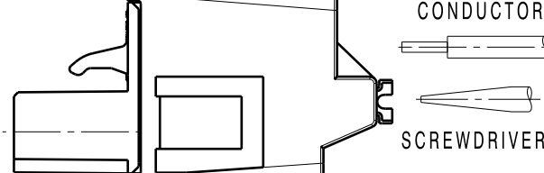
SHOWN: BLF 5.08HC/04/180B
