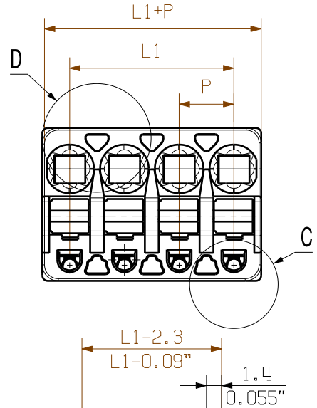
SHOWN: BLF 5.08HC/04/180G
