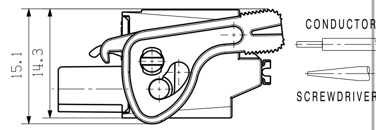
SHOWN: BLF 5.08HC/04/180LR
