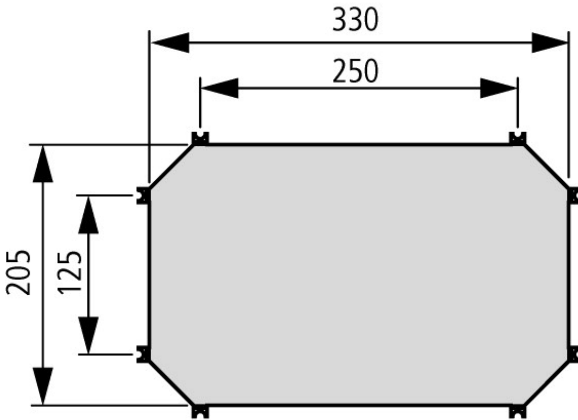
Mounting plate M3-...: 3 mm thick
