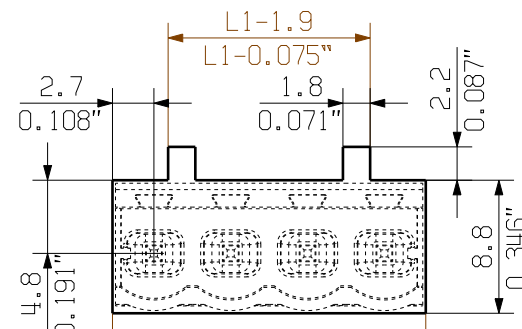
MIN. FRONT PLATE CUT-OUT
