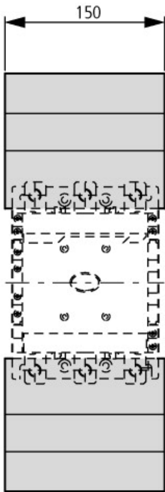
DILM250/300A+DILM...-XHB
