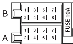
ISO Connector
