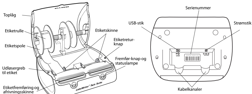
LabelWriter 450 Twin Turbo
