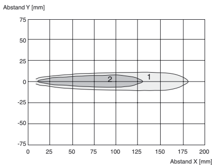
Kurve 1: ebene Platte 10 mm x 10 mm Kurve 2: Rundstab, Ø 8 mm
