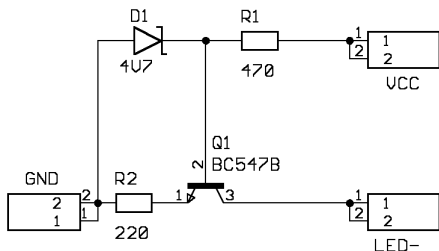
Fig.1: Schaltplan
