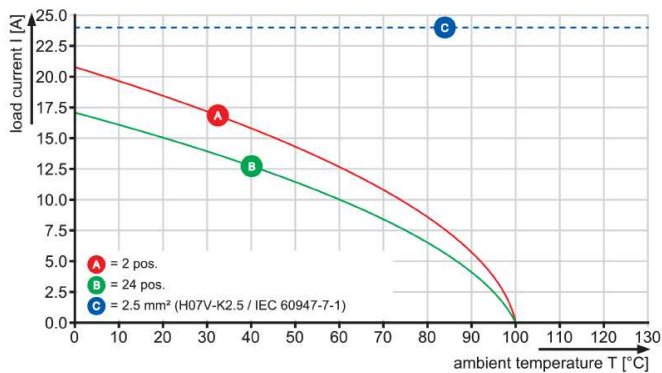
BLT 5.08/..180 - SL 5.08/..90
