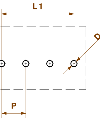
Layout finished holes
