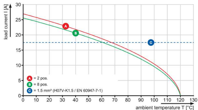
LSF-SMT 5.08/./180 3.5
