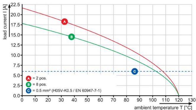
LSF-SMT 5.00/./180 3.5
