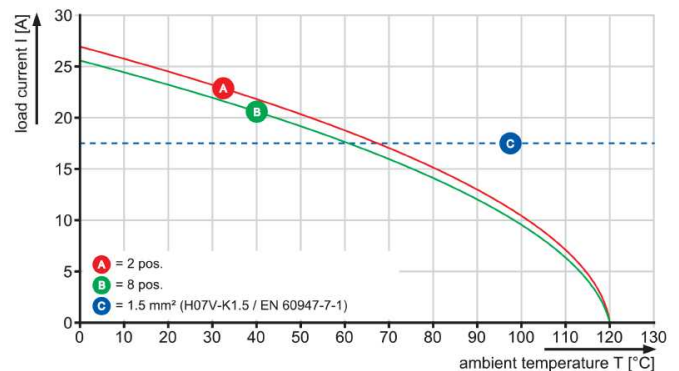
LSF-SMT 5.00/./180 3.5
