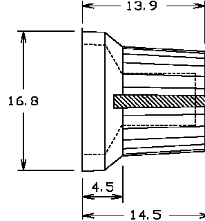
CL170827BR KNOB K87MAR BLACK/BLUE 6mm D
