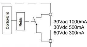
Power Good Relais (Fig.4)
