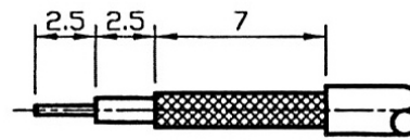
STRIP LENGTHS
