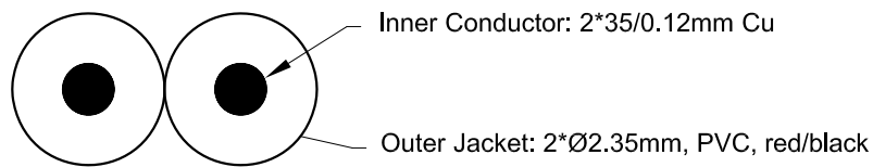
Cable Structure (0.4mm 2 )
