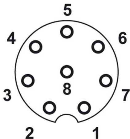
Buchse M12, 8-polig
