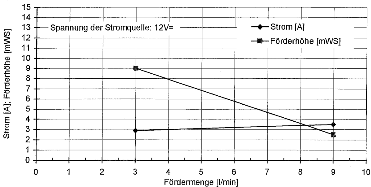
1900.57.00 Tauchpumpe COMET-COMBI 12-2T
