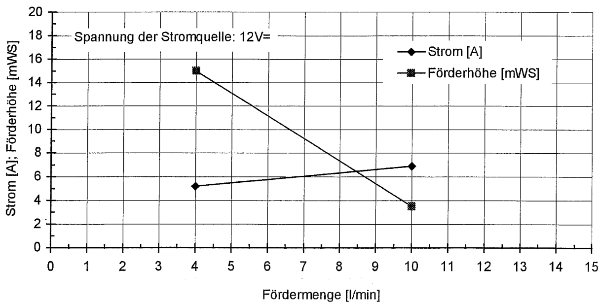
1910.57.00 Tauchpumpe COMET-COMBI 12-4T
