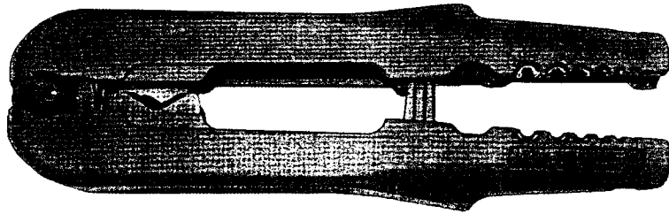
Abmanteln-Abisolieren-Schneiden / Cable stripping-Wire stripping-Cutting
