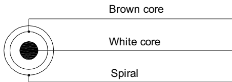
Wire layout
