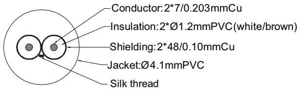
Cable section
