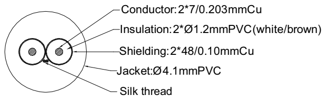
Cable section
