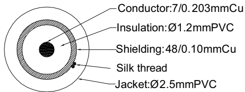
Cable section
