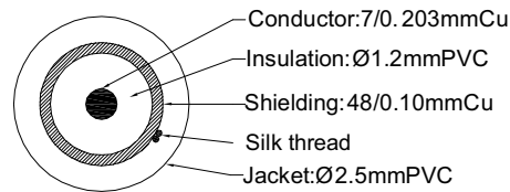
Cable section
