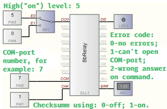
Abb. 5: Profilab-Baustein
