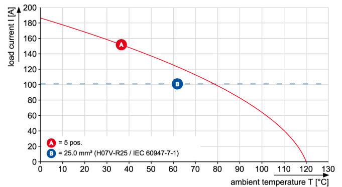
WGK 25 VP
