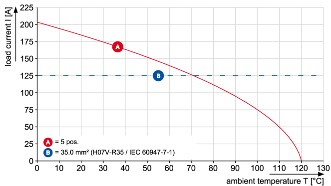
WGK 25 VP
