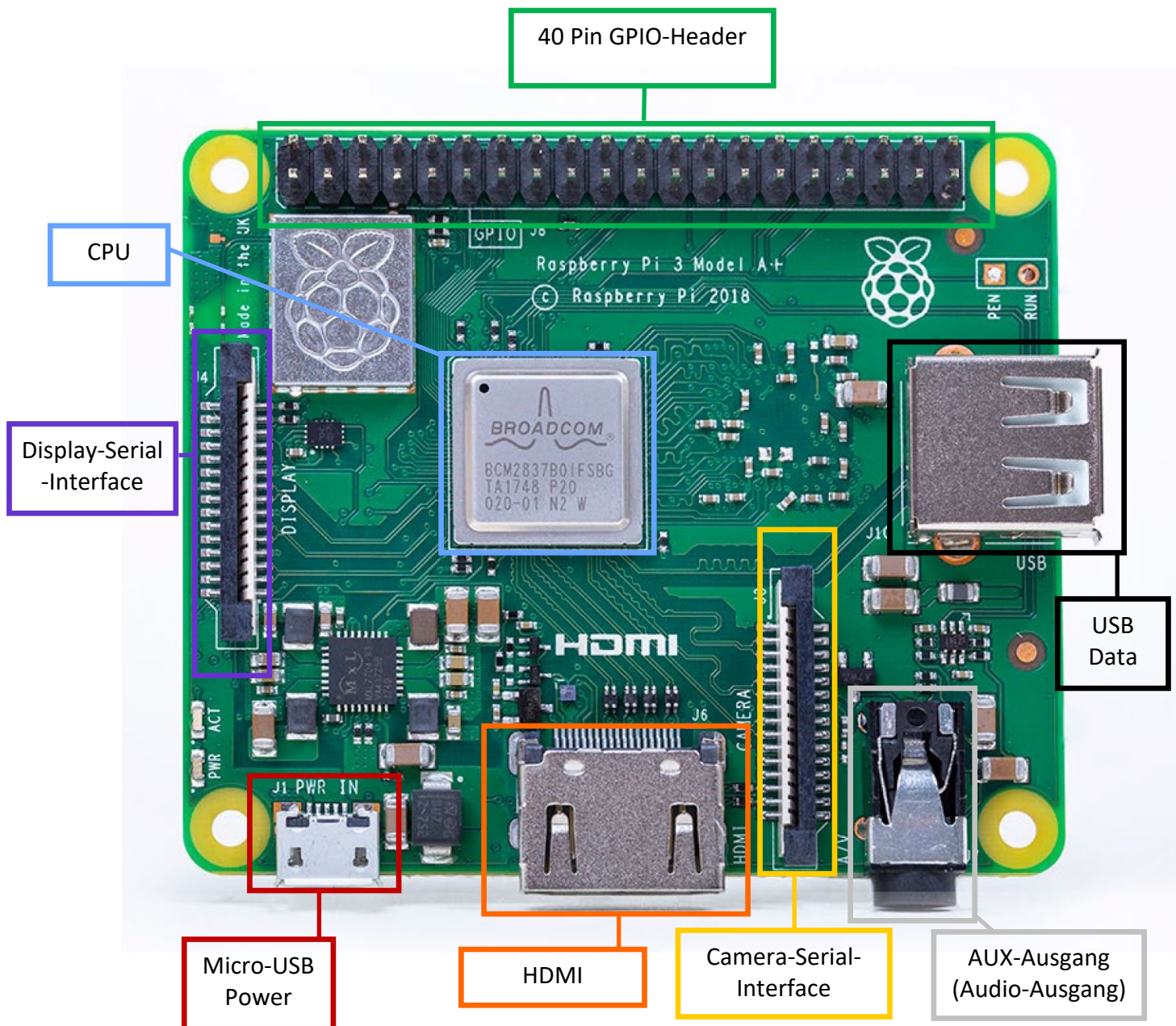
Anschlüsse des Raspberry Pi 3A+
