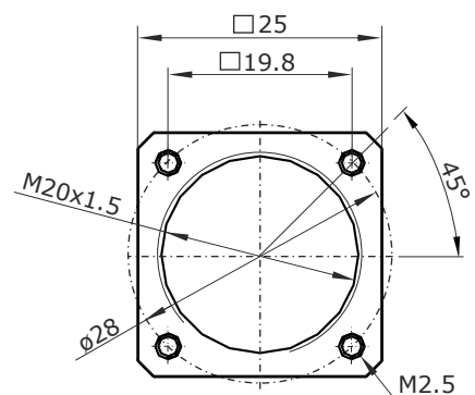
Main Dimensions flange
