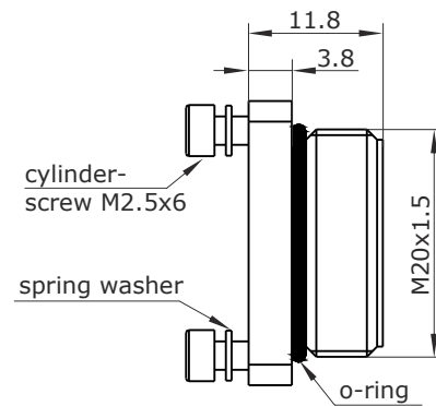
Main Dimensions adapter
