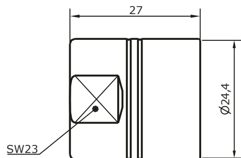
Main Dimensions clamping ring adapter
