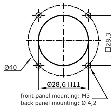
Mounting Hole
