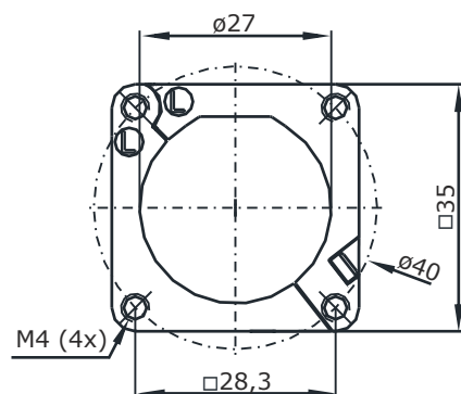
Main Dimensions flange
