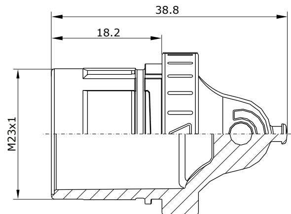
Main Dimensions sealing plug
