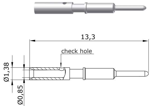
Main Dimensions contact pin
