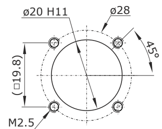
Mounting Hole
