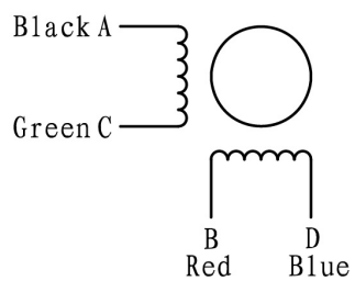
Wiring diagram
