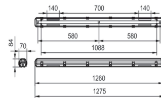
WT050C L1200 1 Tube
