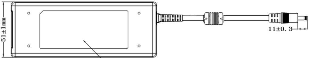
TOP-VIEW
