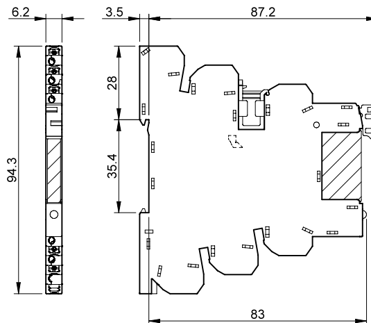
Typ 39.90 39.91 Push-In - Klemmen
