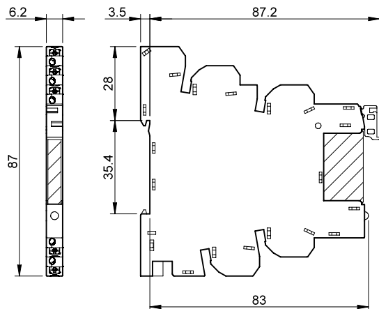
Typ 39.70 39.71 Push-In - Klemmen
