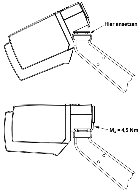
Abb. 1: Speisesystem befestigen
