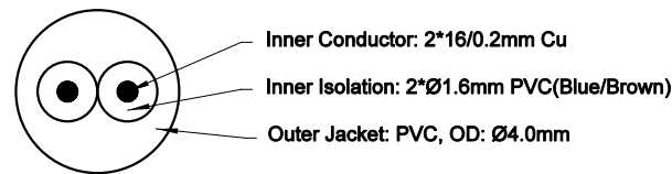
Cable Structure (0.5mm 2 )
