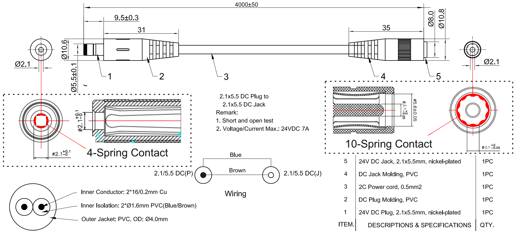
Cable Structure (0.5mm 2 )
