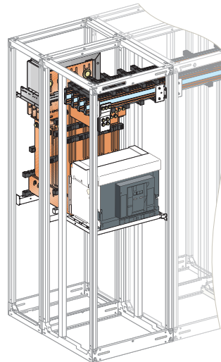
Connection using Canalis busbar trunking.
