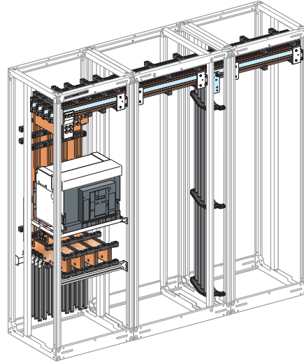
P4000 switchboard with front connection.
