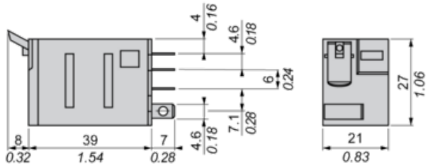
Pin Side View
