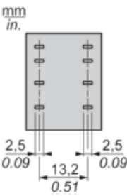
Pin Side View
