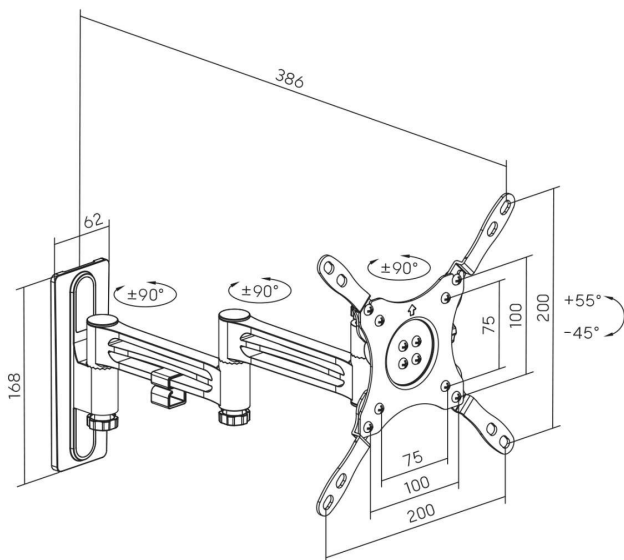
Dimensions (mm)
