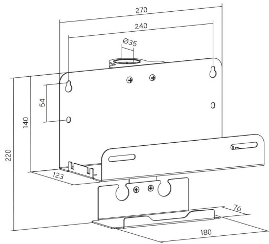
Dimensions (mm)
