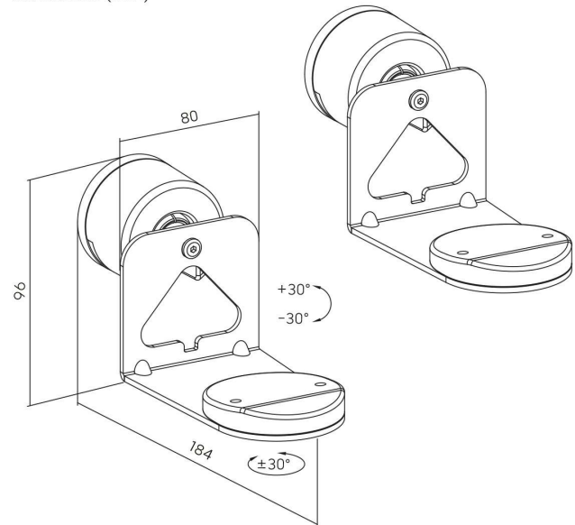
Dimensions (mm)
